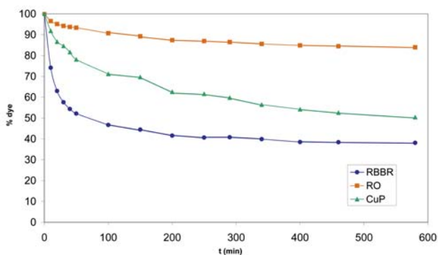
Figure 3. Decolourisation of three different dyes: Reactive Orange 16 (RO16) Remazol Brilliant Blue R (RBBR) and Copper(II) phthalocyanine (CuP) with enzyme mixtures obtained on beech wood (Lac 1550 U/L) and MnP (70 U/L)
